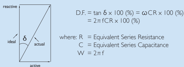
Fig. I-6 The \tan \delta is measured with the same set up as for the series capacitance ESC
